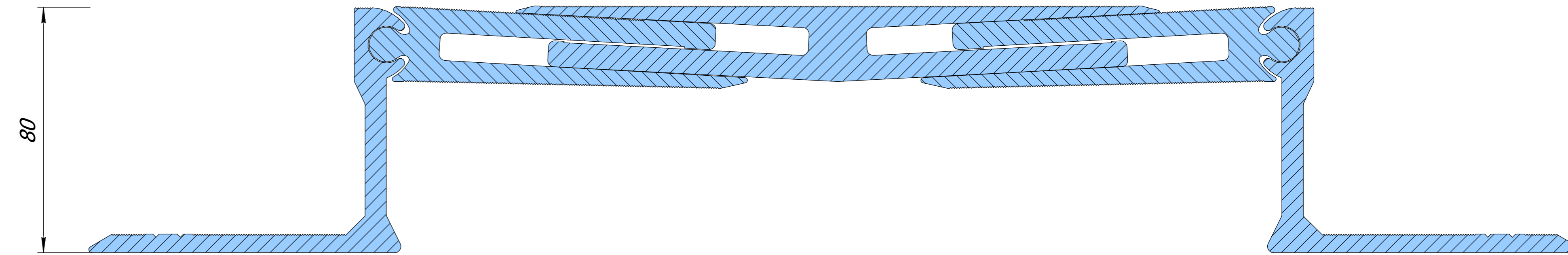
Dewmark Heavy SV 45/300/80
